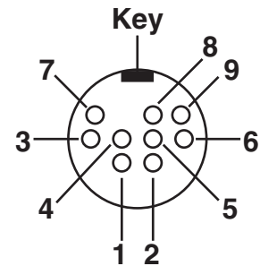
9 pin Mini-Din male motor connector (front view)
